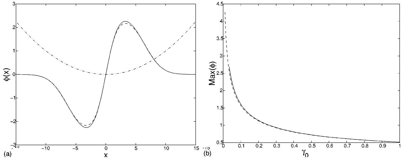
FIG. 1. (a) Example of a dark soliton solution for \omega=-0.5 , \Omega^2=0.02 , \gamma_0=0.1 , and \gamma_1=2.5\sqrt{\gamma_0} . The dashed curve shows the result from Eq. (10) and the solid curve shows the result from Eq. (11) of [2]. The potential is shown by the dashed-dotted line. (b) Continuation branch of dark soliton solutions as a function of \gamma_0 for the same parameters.
