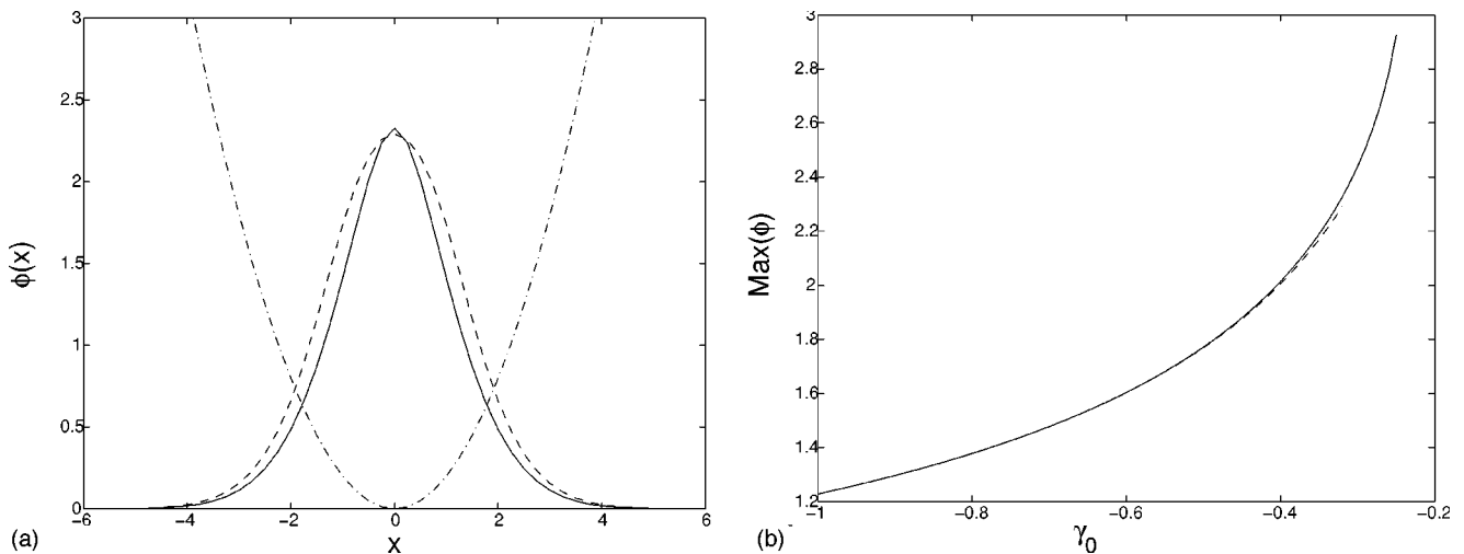
FIG. 2. Same as in Fig. 1, but for a bright soliton solution branch. The case of \omega=0.5 , \Omega^2=0.4 , \gamma_0=-0.32 , and \gamma_1=1 is shown in the left panel.
